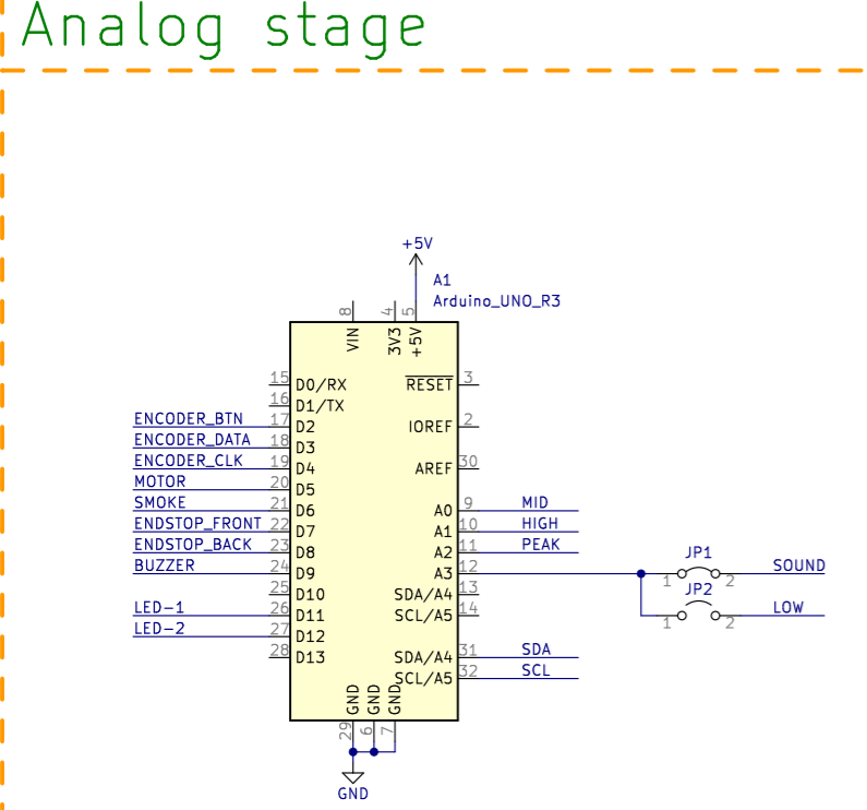
Arduino connector
