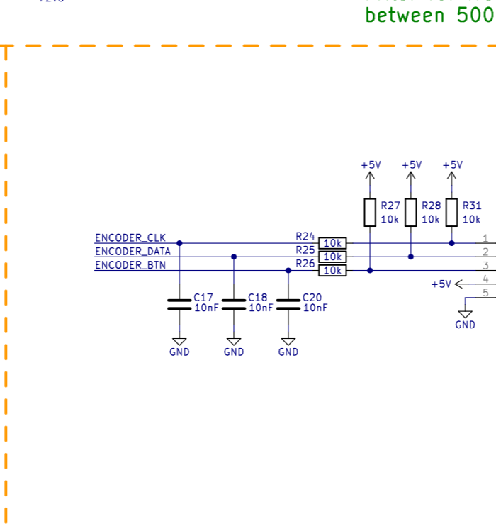
Encoder interface
